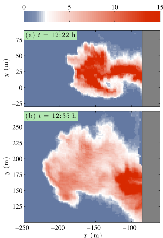
Figure 14. Aerial multispectral images of inner-shelf surface dye concentration D (ppb, see color bar) versus cross-shore coordinate x and alongshore coordinate y for (a) a transient rip current ejection event at t=12:22 h and (b) the subsequent dye evolution at t=12:35 h approximately 150 m downstream. Gray denotes the surfzone, largely unresolved in the aerial imagery due to foam from wave breaking. The near-shoreline dye release is at (x, y) = (-10, 0) m.
