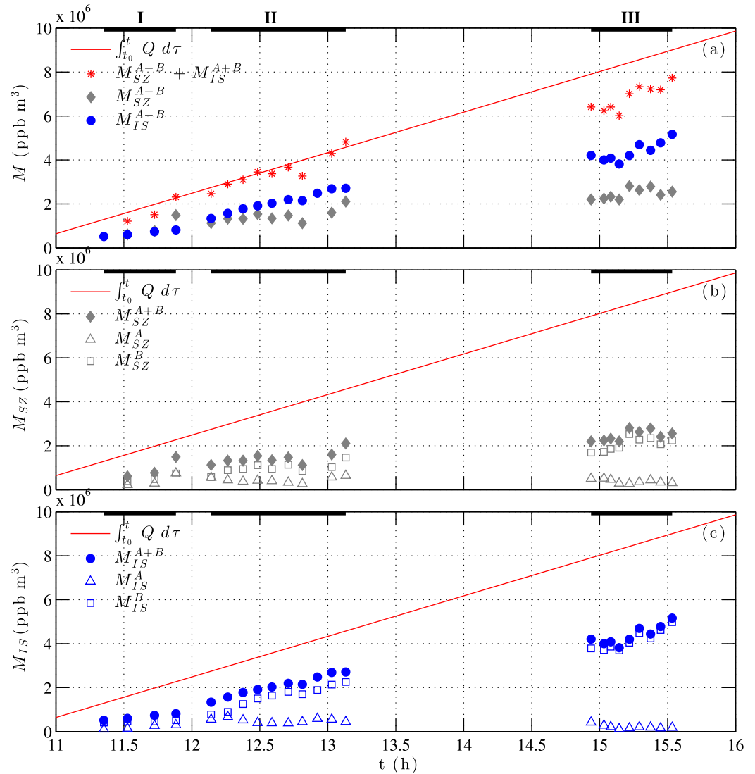
Figure 8. Dye mass M versus time. Black bars denote time periods I, II, and III. (a) Surfzone estimates M_{SZ}^{A+B} (gray) are from in situ observations, and inner-shelf estimates M_{IS}^{A+B} (blue) are from aerial observations. Red asterisks are M_{SZ}^{A+B} + M_{IS}^{A+B} . Red line shows the time-integrated dye mass released since t_0 = 10:39 h ( \int_{t_0}^t Q d\tau , where Q is the steady dye release rate). (b) Surfzone dye mass M_{SZ} versus time for the near-field region A ( y \leq 248 m, triangles) and the far-field region B ( y > 248 m, squares). Solid gray diamonds are M_{SZ}^{A+B} . (c) Inner-shelf dye mass M_{IS} versus time for region A (triangles) and region B (squares). Solid blue circles are M_{IS}^{A+B} . Estimation methods for M_{SZ} and M_{IS} are described in Appendices A1 and A2, respectively.
