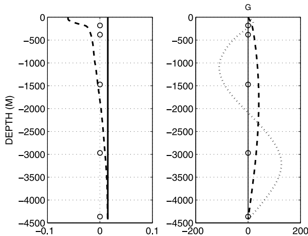
Fig. 6. Instrument depths (mooring A) superimposed upon the horizontal velocity/pressure modes, F_i , i = 0,1 , (left-hand side) and vertical displacement modes, G_i , i = 0,1,2 for a flat-bottom, resting ocean, subject to a rigid lid surface boundary condition. The sharp increase in the amplitude of the F_1(z) mode near the surface, z = 0 , is an important characteristic, but is poorly defined by the available instrumentation. The barotropic vertical displacement mode is plotted as zero amplitude.
