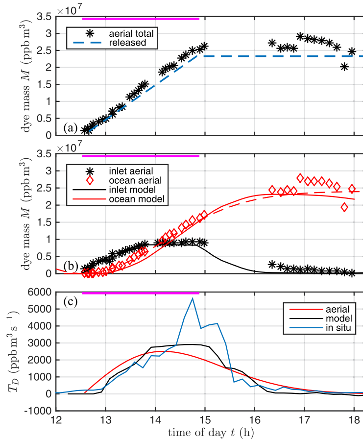
Figure 11. (a) Total (inlet + ocean) aerial-observed dye mass M_{\text{tot}} (black asterisk) and total released dye (blue dashed) versus time. The total dye released M_{\text{rel}} = 2.33 \times 10^7 ppb m³. (b) Ocean M_{\text{oc}} (red) and inlet M_{\text{in}} (black) dye mass versus time for aerial-observed (symbols) and modeled (curves). The best fit functional form (13) aerial-observed ocean M_{\text{oc}}^{(\text{obs})} is given by the red dashed curve. (c) Dye transport T_D from inlet to ocean versus time for the in situ (blue), aerial observed (red), and model (black). In all figures, the magenta bar indicates the duration of the dye release.
